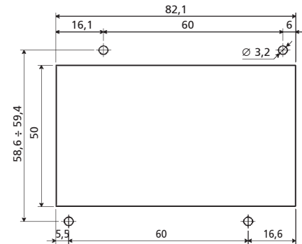
Drilling template
