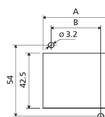
Drilling template
