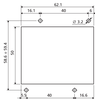
Drilling template
