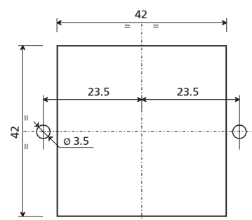
Drilling template
