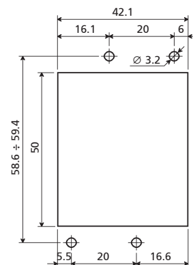
Drilling template
