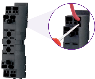
Ressort
