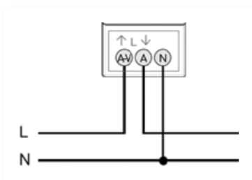
Tariff inputs & S0 pulse outputs
