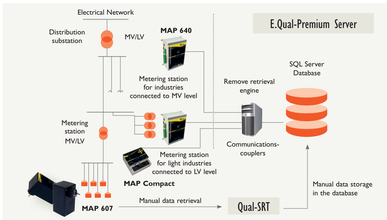
Components of an E.Qual-Premium Server with the network analyzers, the communication links, the database and the analysis and graphic display modules.
