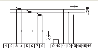
TD320 configuration
