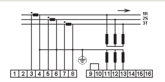
TD320Y configuration
