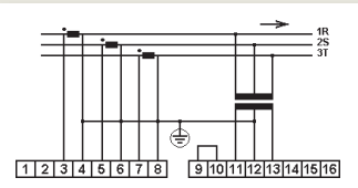
TD320D configuration
